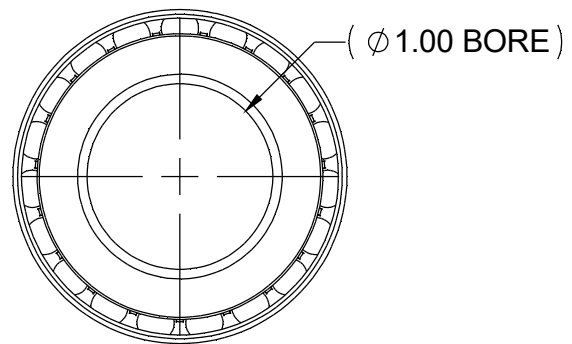
2X X000-4300-F0178 CONES USE WITH X000-4300-F0177 RACES
