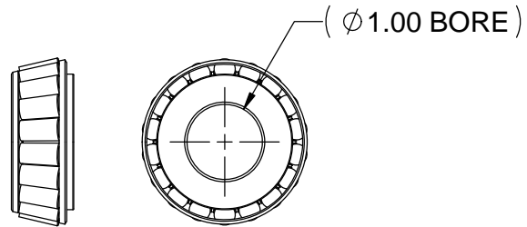
2X X000-4300-H0140 CONES (USE ON THE INPUT SHAFT)
