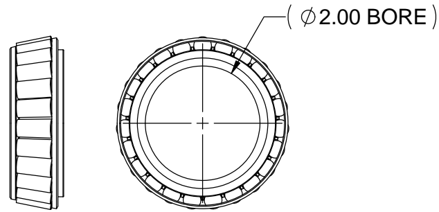
2X 804949 CONES (USE ON THE OUTPUT SHAFT)
